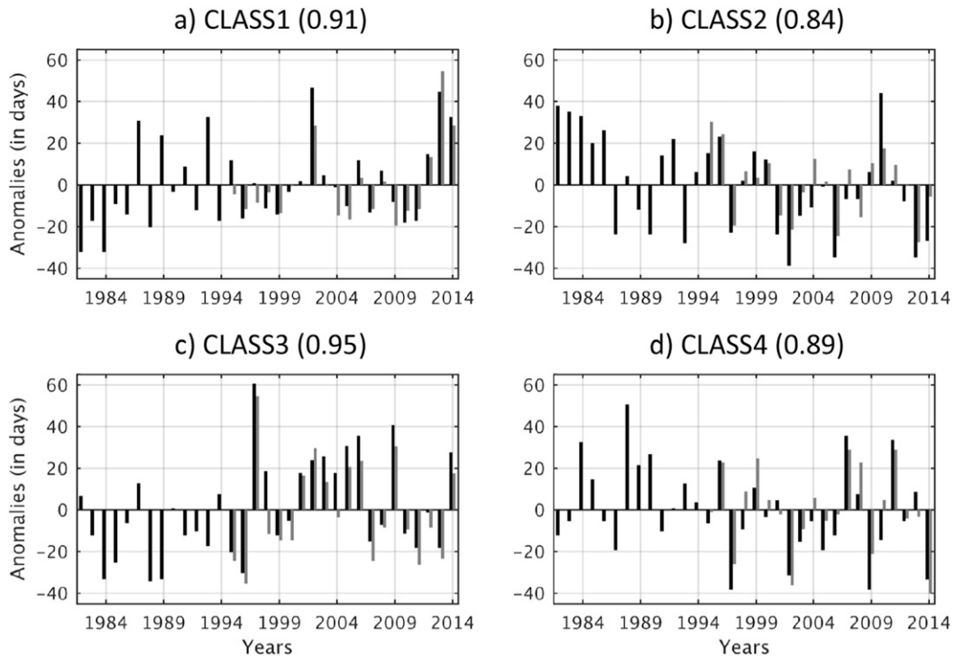
FIG. 8. Yearly regime occurrence anomalies for MERRA (black) and ECMWF week 1 (gray) per October–March seasons during the 1982–2014 and 1995–2014 periods, respectively. Correlations between both time series over the 1995–2014 period are indicated in the title of each panel and are all significant at 1% significance level using Monte Carlo simulations.
